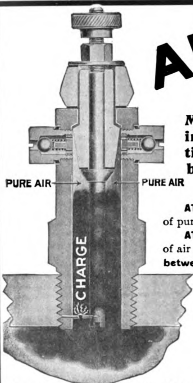
Note the relative position of insulation, pure air, charge, and spark at the instant of explosion.
